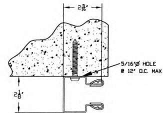
CONCRETE/FILLED BLOCK JAMBS USING 5/16" X 2-1/4" TAPCON XL
