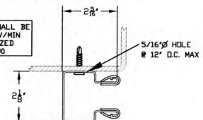
STEEL JAMBS USING #12-14 X 1" TEKS PANCAKE HEAD 16 GA (.063) GUIDE MOUNTING DETAIL
