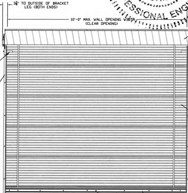
INSIDE ELEVATION
