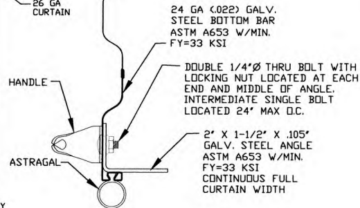
BOTTOM BAR ASSEMBLY
