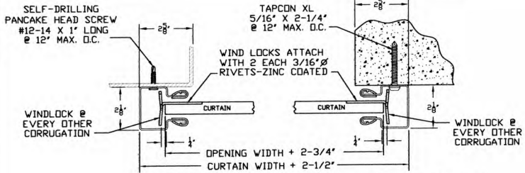
STEEL JAMBS LH GUIDE MOUNT SHOWN
